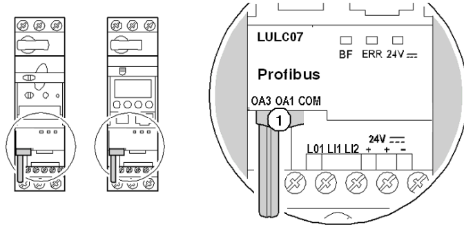
1 Link for connecting outputs OA1 and OA3 to terminals A1/A3/A2 on the starter.
