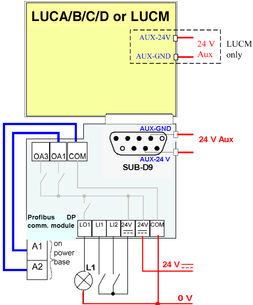
Schematic of the 24 V \equiv and the 24 V Aux power supplies
