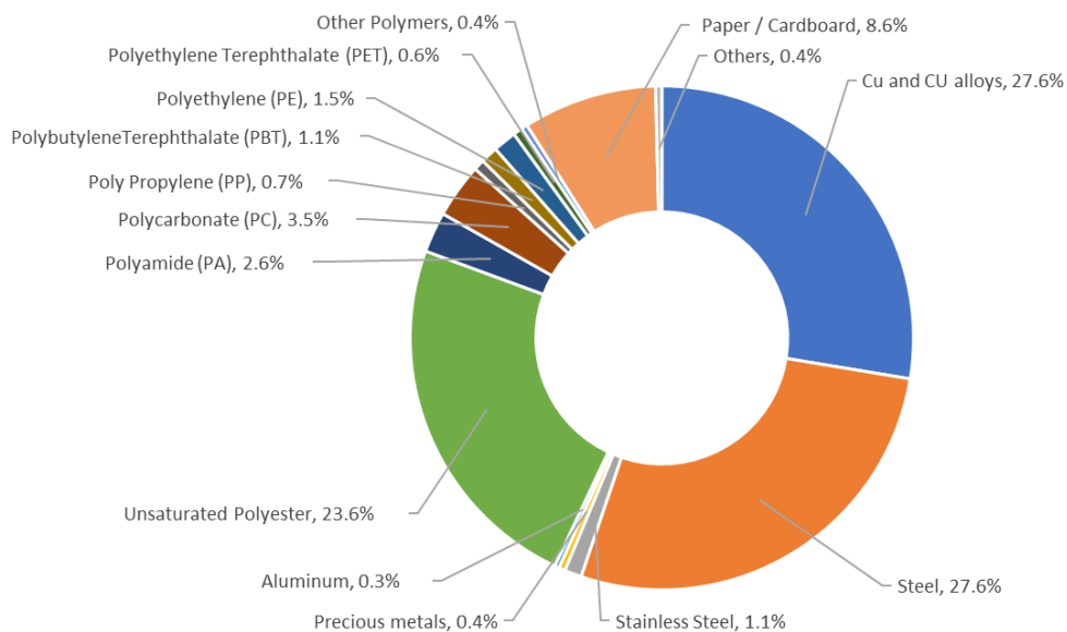
Figure 1: Composition of XT7M 1600A L - 3P IEC
