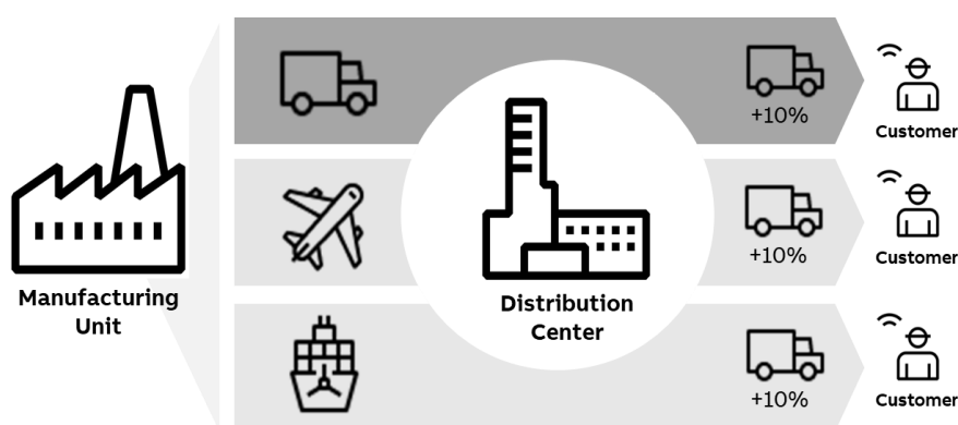
Figure 4: Distribution methodology.
