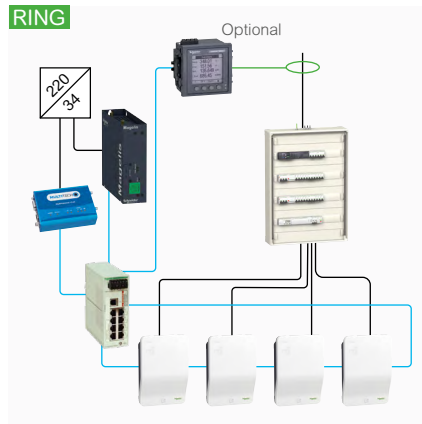
Ring connection with manageable switch part number TCSEBU083F23F0 or TCSELU043F23F0
