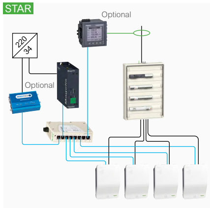
Star connection using basic switch part number TCSEU083FN0. Non manageable
