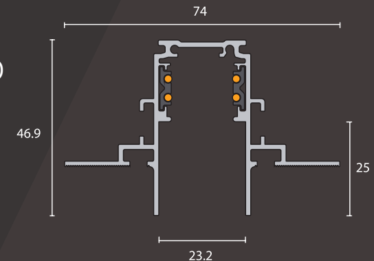
RECESSED TRACK
