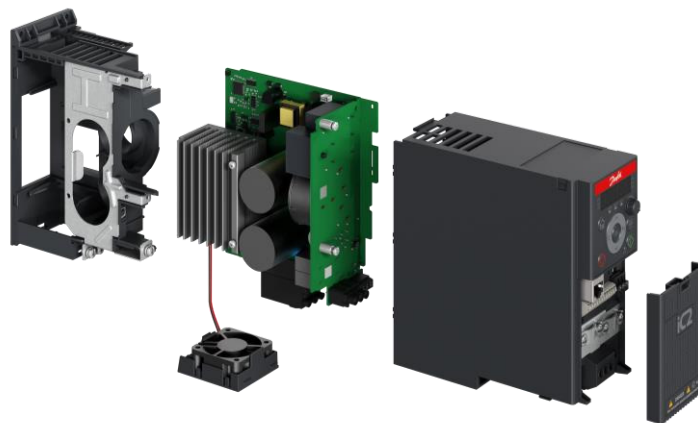
Figure 1: Exploded view of the iC2-Micro Frequency Converter, Frame size MA02a.
