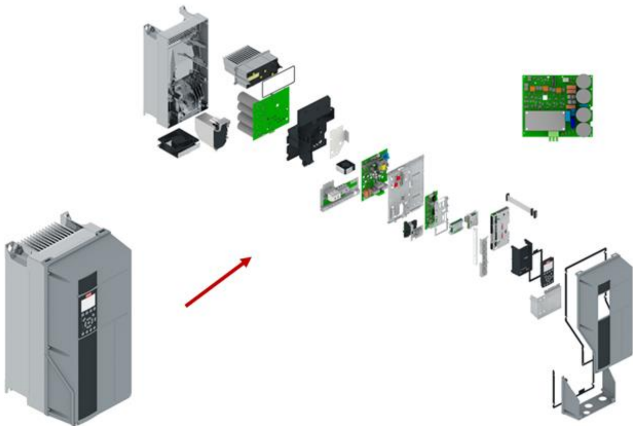
Figure 1: The exploded illustration of the drive with its main components.
