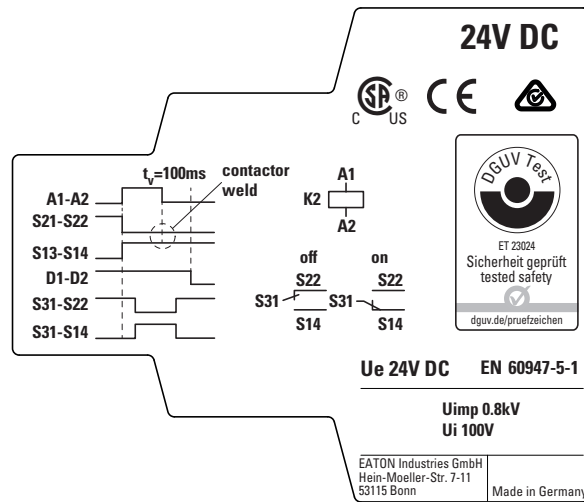
Figure 6: Nameplate
