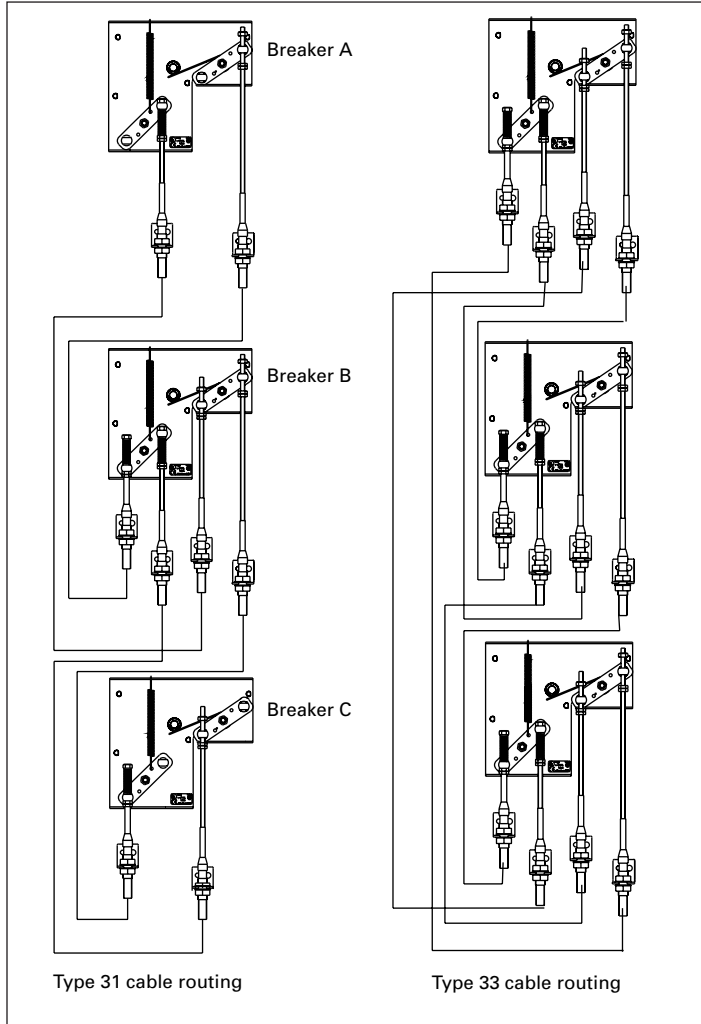
Figure 11. Cable routing for Type 31 and 33 interlock configurations
