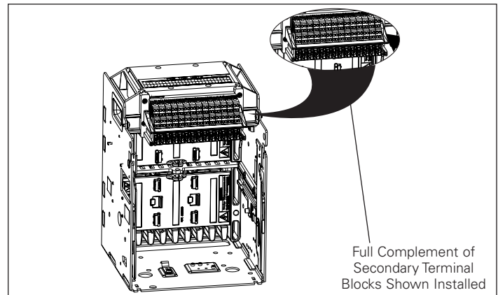
Figure 11. Cassette-Mounted Terminal Blocks NF Frame.
