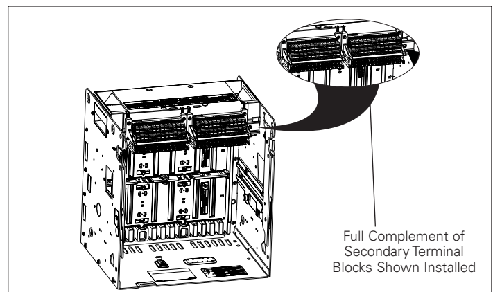
Figure 11A. Cassette-Mounted Terminal Blocks RF Frame.
