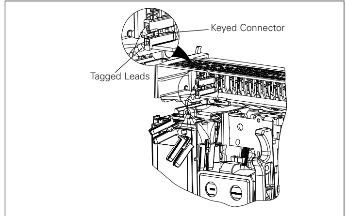
Figure 3. Leads and Connectors (Drawout Configuration Shown).
