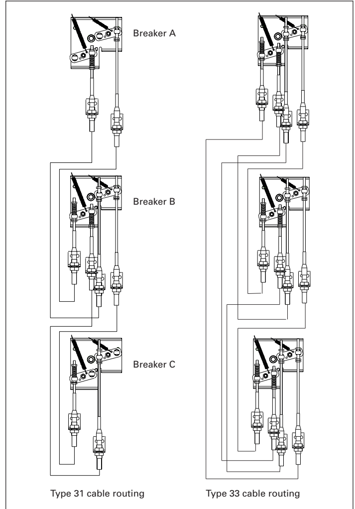
Figure 1. Cable routing for Type 31 and 33 interlock configurations
