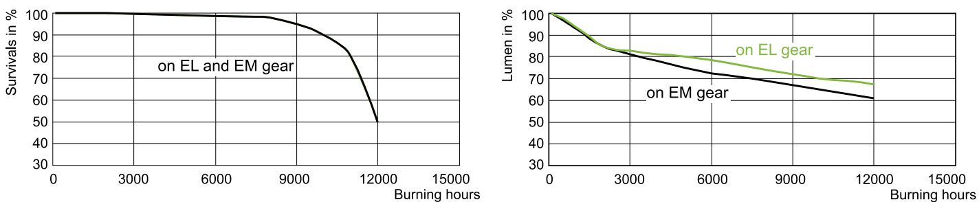
LDLE_CDM-T_150W_942-Life expectancy diagram
