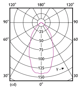
LEDspot CorePro 1.8-30W E14 R39 827 36D ND
