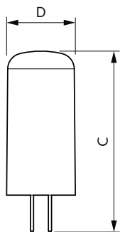
CorePro LEDcapsuleLV 2.1-20W G4 827 D
