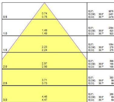
Distance [m] Cone diameter [m] C0 - C180 (Half beam angle: 73.4°) C90 - C270 (Half beam angle: 73.2°)
