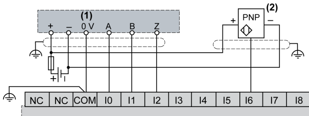
(1) Dual phase encoder with index (2) PNP sensor
