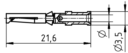
female contact
