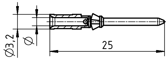
male contact
