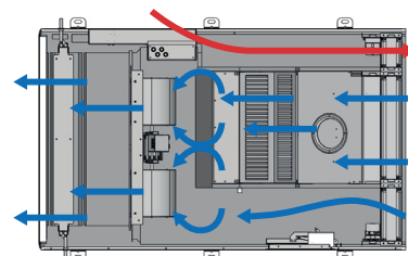
Fresh air is supplied to the room passively via other openings such as windows and is assisted by the NVHRe unit to distribute the air effectively throughout the room and further enhance occupants' comfort.
