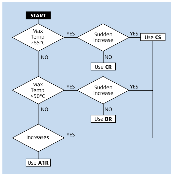
Fig. 3 Choosing a heat detector
