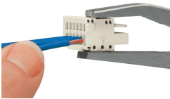
Inserting a conductor via operating tool.
