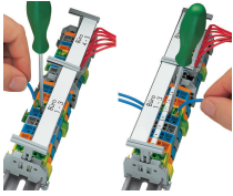
Laterally movable marking system
