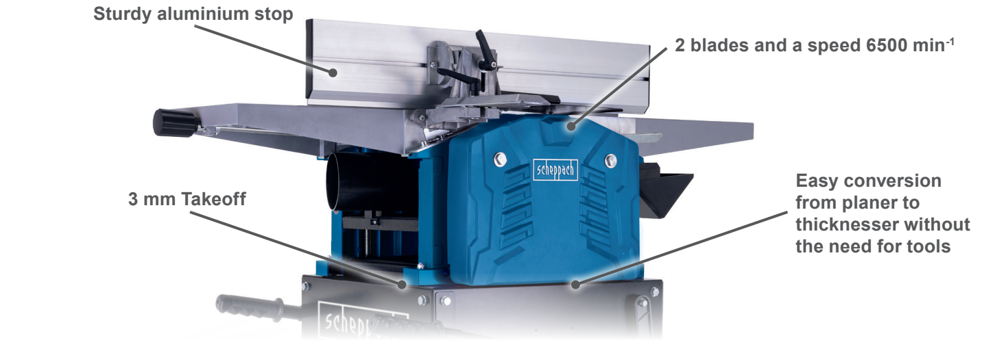
2 high-speed steel planer knives, blade speed 6500 rpm for smooth and precise planing.
