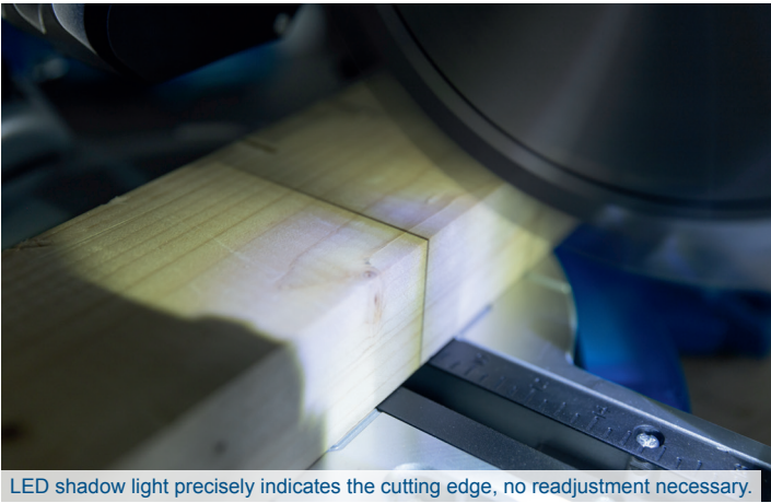
LED shadow light precisely indicates the cutting edge, no readjustment necessary.
