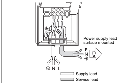
Power supply lead flush fitted
