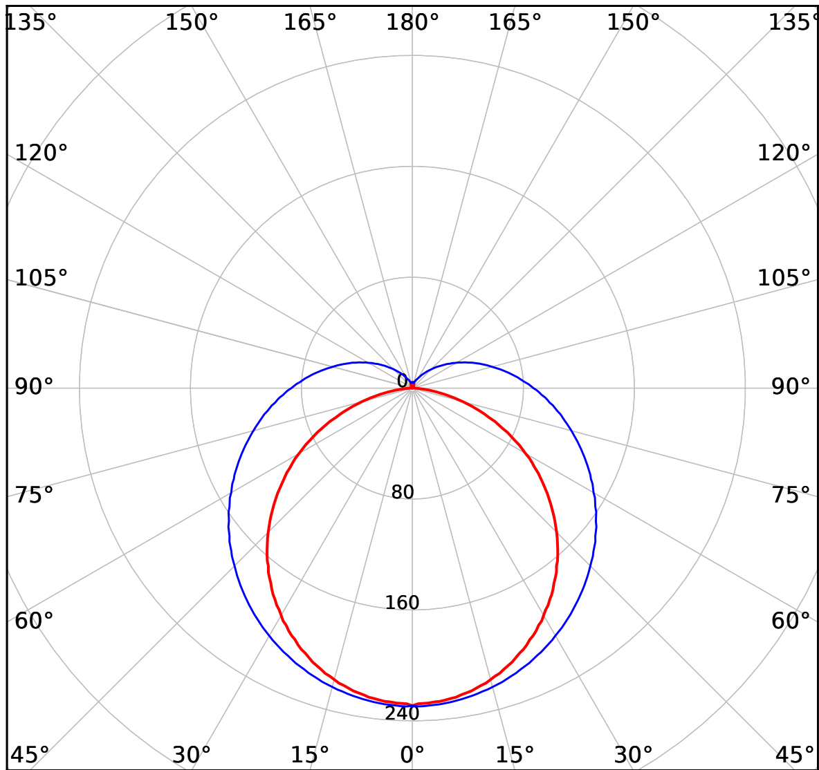
cd 950 lm — C0-C180 — C90-C270
