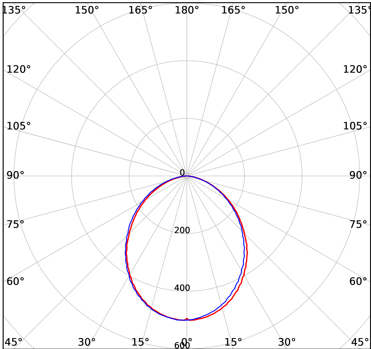
cd 1200 lm — C0-C180 — C90-C270
