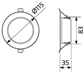
LEDDownlightCo-E Rd100
