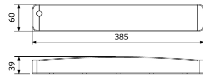
LEDPanelSp-Z Driver
