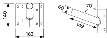
LEDStreetlight Wall-Bracket-60
