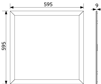
LEDPanelRc-S5 Sq595
