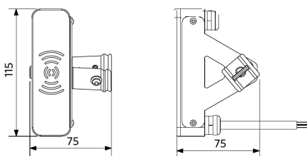
LEDflood-E Sensor
