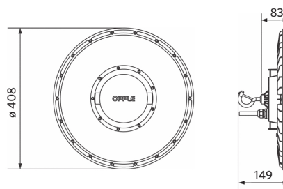
LEDHighbay-P5 Reflector-D420
