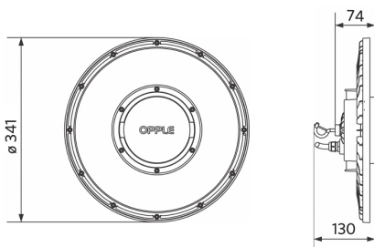
LEDHighbay-P5 Reflector-D330
