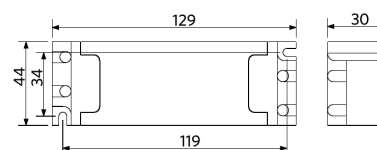
LEDPanelRc-S-E2 Driver
