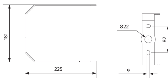
LEDHighbay-P5 Bracket-D420
