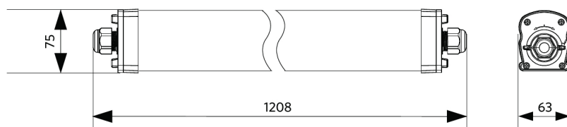
LEDWaterproof-P4 L1208
