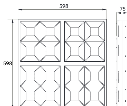
LEDPanelRc-G Sq598
