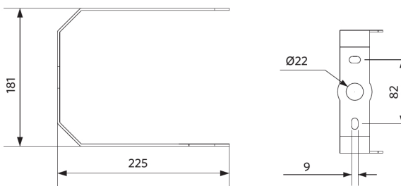
LEDHighbay-P5 Bracket-D420
