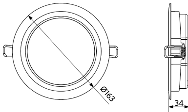
LEDDownlightRc-SI-E Rd150
