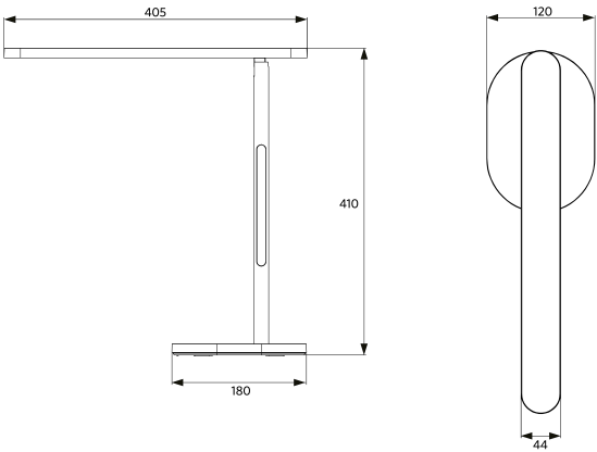
LEDSparrow-E
