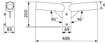
LEDStreetlight Pole-Top-60-Adapter-2x60
