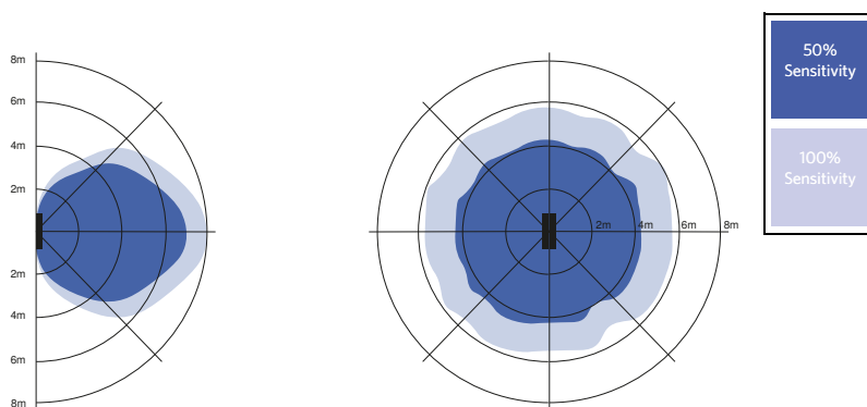
Installation - Wall mounted Suggested installation height 1-3m
