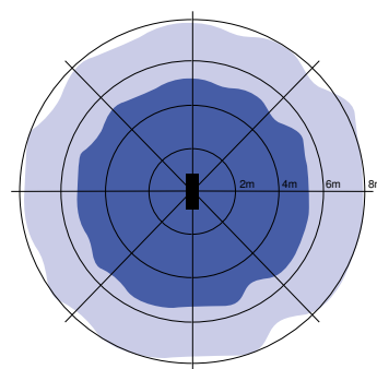
Installation - Ceiling mounted Suggested installation height 2.5-10m
