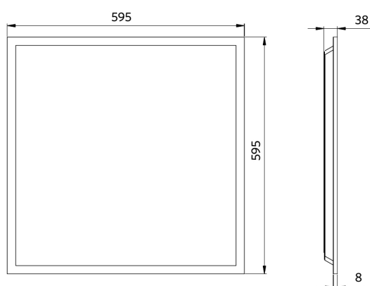
LEDPanelS-B3 Re295-32W
