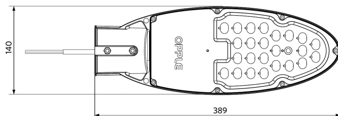
LEDStreet-SE-ExtensionCable
