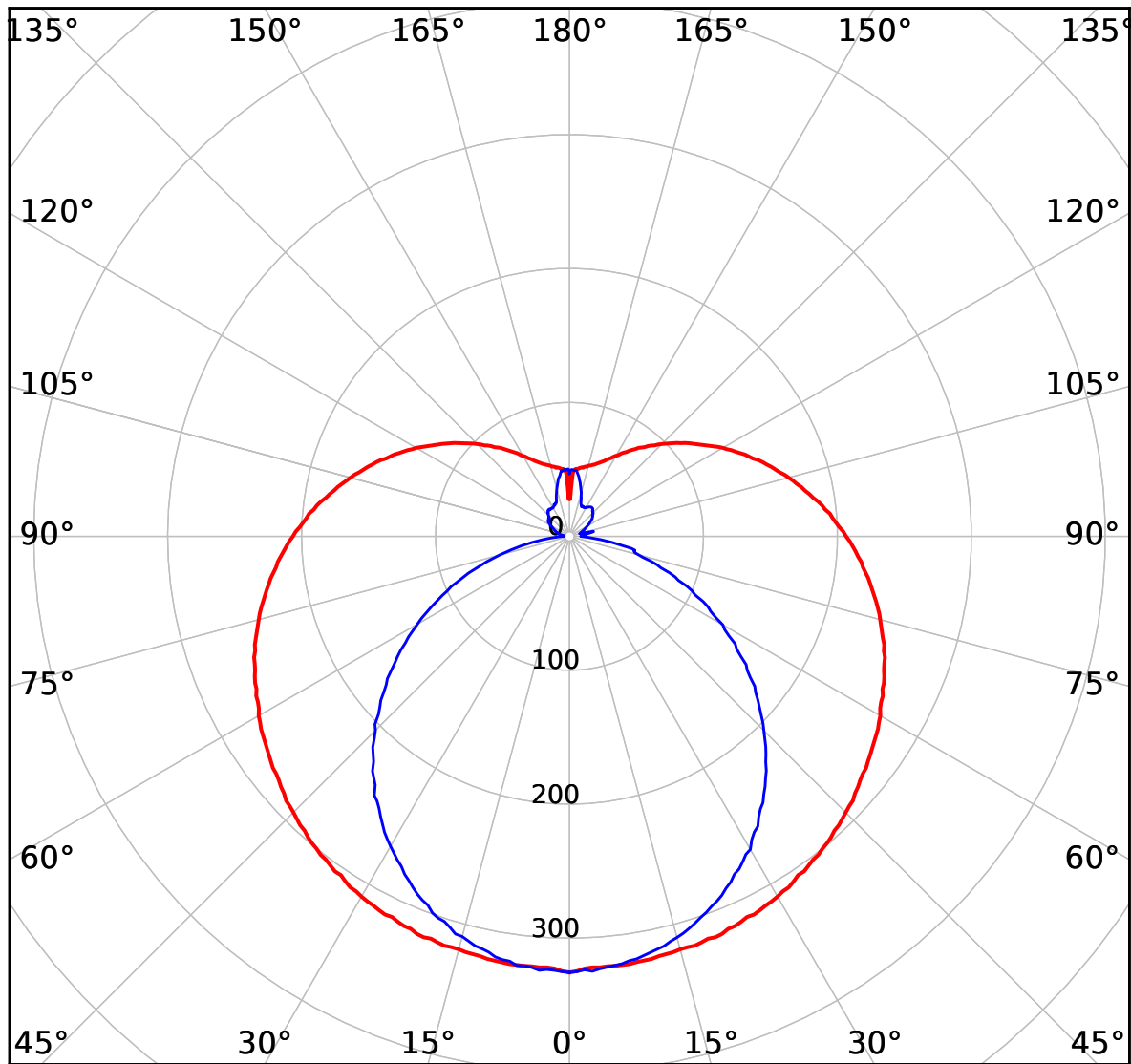
cd 1800 lm — C0-C180 — C90-C270
