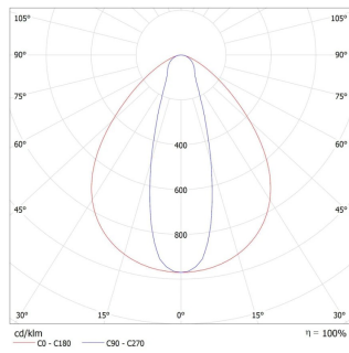
OPPLE 545001108600 LED HB-Lin-P 240W-DALI-XAS / LDC (Polar)
