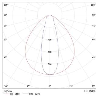
OPPLE 545001108700 LED HB-Lin-P 300W-DALI-XAS / LDC (Polar)
