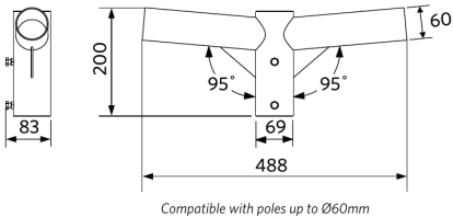
LEDStreetlight Wall-Bracket-60
