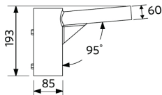
LEDStreetlight Pole-Top-76-Adapter-60
