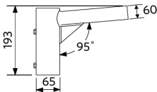
LEDStreetlight Pole-Top-60-Adapter-60
