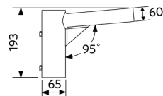
LEDStreetlight Pole-Top-60-Adapter-60
