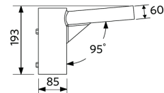
LEDStreetlight Pole-Top-76-Adapter-60
